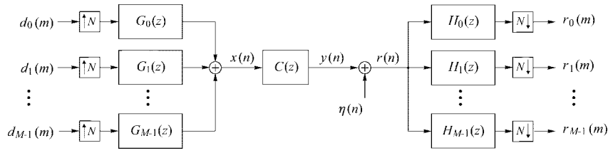
Fig. 1. Transmultiplexer with transmission channel and additive noise.
